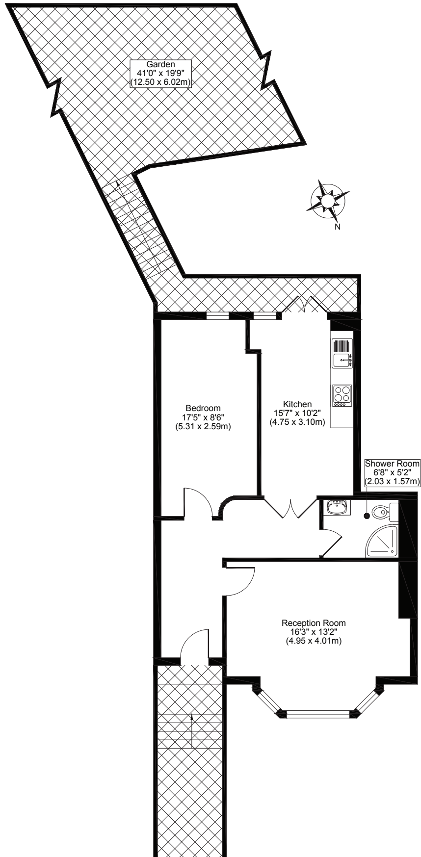
RAISED GORUND FLOOR
