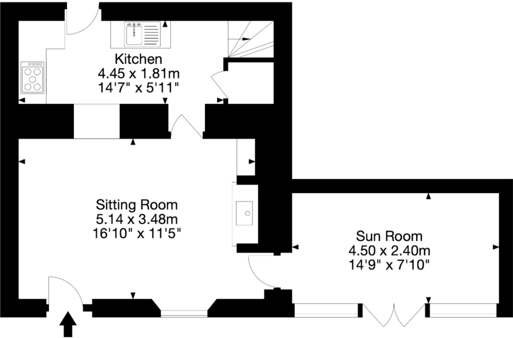
Ground Floor
